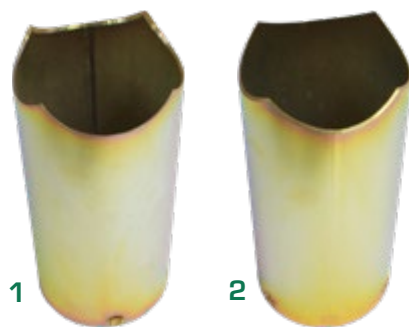
1. Inside Edge Scalloped Blade [No. 220-IN] 2. Outside Edge Scalloped Blade [No. 220-OUT]
